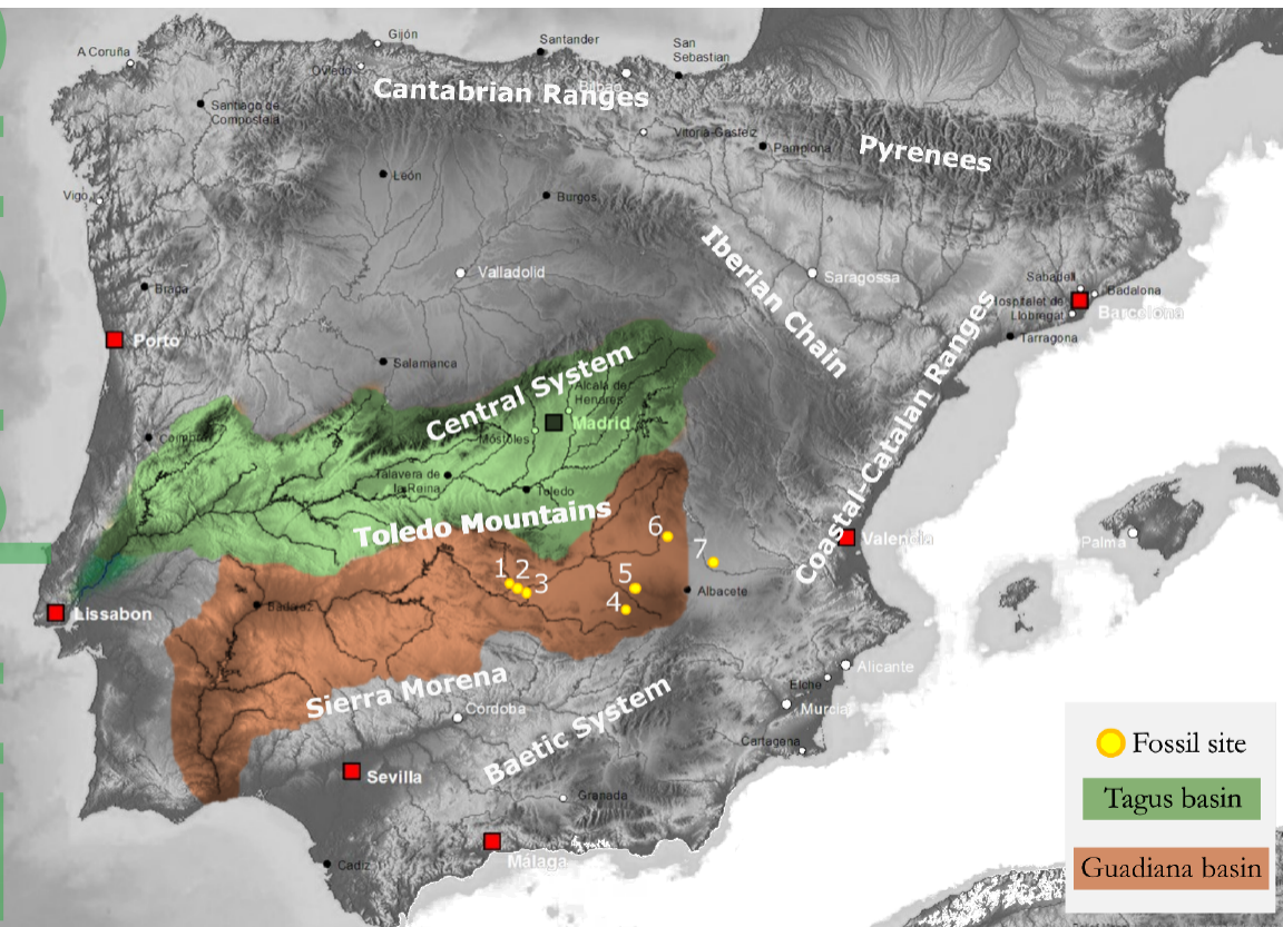
Figure 1: Geographical setting of the Tagus (green) and Guadiana (brown) Basins. The main fossil sites identified in the Upper Guadiana basin (yellow circles) are highlighted. 1: Bonete y Piedrabuena (Pliocene); 2: Las Higuieruelas (Pliocene); 3: Valverde de Calatrava I (Lower to Middle Pleistocene) and II (Pliocene); 4: Cueva de los Toriles (Middle Pleistocene); 5: Los Villares (Middle Pleistocene); 6: El Provencio (Middle Pleistocene); 7: Fuensanta del Júcar (Lower to Middle Pleistocene). Modified from https://commons.wikimedia.org/ , CC BY-SA 3.0.
